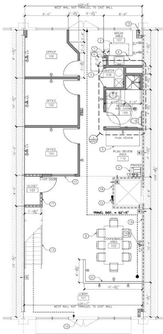
1 FLOOR PLAN - FIRST FLOOR SCALE: 1/4" = 1'-0" AREA: 1,481 SF
