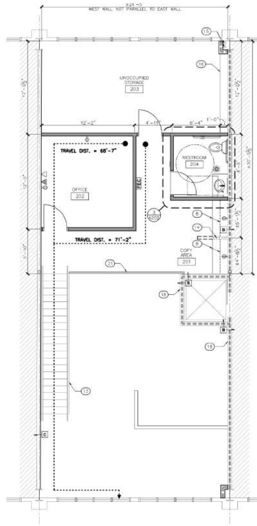
1 FLOOR PLAN - SECOND FLOOR SCALE: 1/4" = 1'-0" AREA: 774 SF
