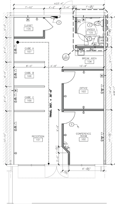
1 FLOOR PLAN - FIRST FLOOR
