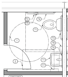
3 ENLARGED RESTROOM PLAN
